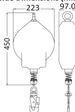
Side Dimensions (mm)
